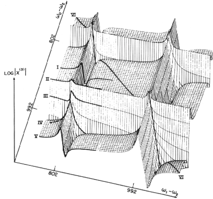
Figure 9. (from reference [28]) Two-dimensional plot of the dispersion of |\chi_{1111}^{(3)}|^2 versus the two difference frequencies in a 1:1 mixture of benzene and cyclohexane. The heavy lines show data obtained by FWM and path VI corresponds to CARS. The ratio of the Raman cross sections of benzene and cyclohexane was determined from such plots to be 3.45:1.
